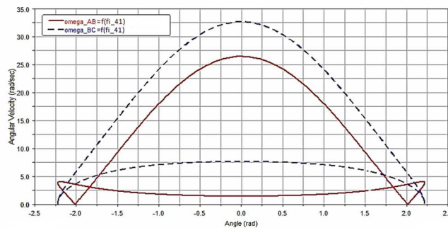
Fig. 10. The angular velocity \omega_{AB} = f(\varphi_{41}) and \omega_{BC} = f(\varphi_{41})
