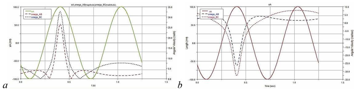
Fig. 8. Displacement x_A = f(t) , magnitude of angular velocity \omega_{AB} = f(t) and \omega_{BC} = f(t) (a); displacement x_A = f(t) , angular velocity \omega_{AB} = f(t) and \omega_{BC} = f(t) (b)
