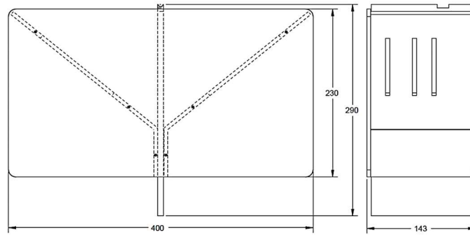
Fig. 7. V-shaped hopper
